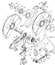
Connector, Guard TS 410
