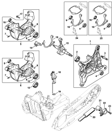
Crankcase
