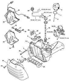
Tank housing
