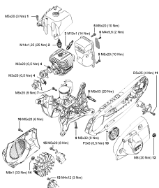
Tightening torques
