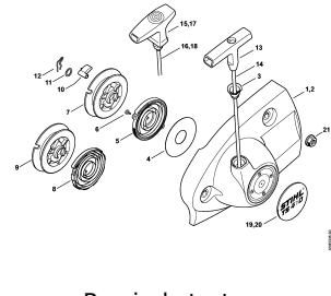
Rewind starter
