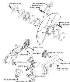
Tightening torques
