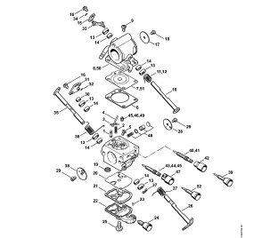
Carburetor C1Q-S118, C1Q-167
