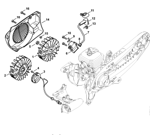
Ignition system
