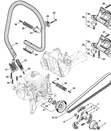
Clutch, Handlebar
