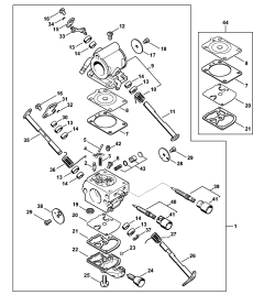
Carburetor 4238/03
