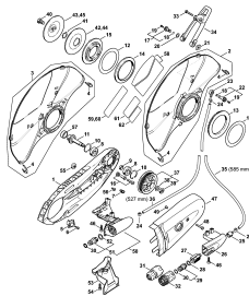
Connector, Guard TS 420
