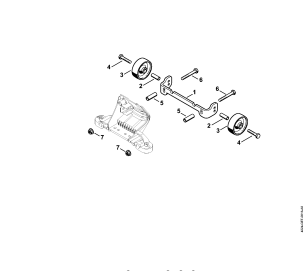
Wheel kit
